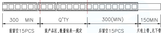
DETAIL A
