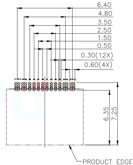
RECOMMENDED PCB LAYOUT(TOP VIEW) THICKNESS 0.60MM;DEFAULT TOLERANCE:±0.05
