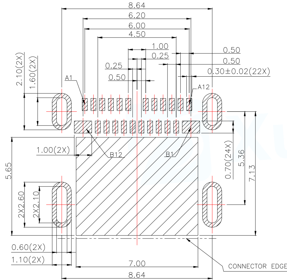
RECOMMENDED PCB LAYOUT(TOP VIEW) DEFAULT TOLERANCE:±0.05
