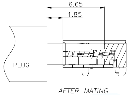
AFTER MATING
