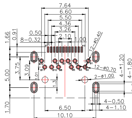
RECOMMENDED PCB LAYOUT Tolerance:±0.05mm
